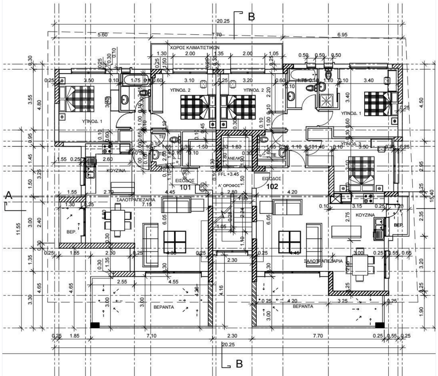
ΚΑΤΟΨΗ Α' ΟΡΟΦΟΥ
