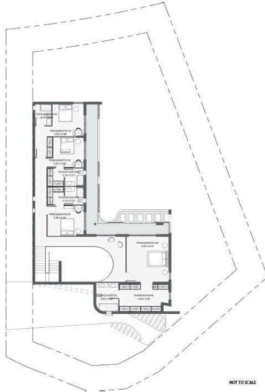
FLOOR PLANS - FIRST FLOOR
