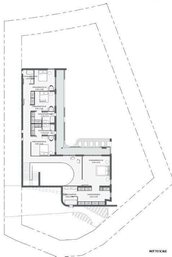
FLOOR PLANS - BASEMENT
