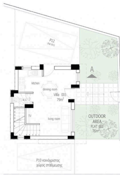
Ground Floor Plan for Villa
